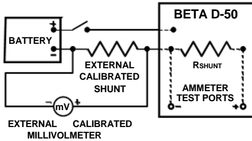
Figure 5-3 Circuit diagram for shunt verification
